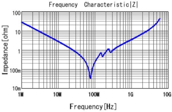
■ GRM3195C2A562JA01 |Z| DCOV, 25degC
