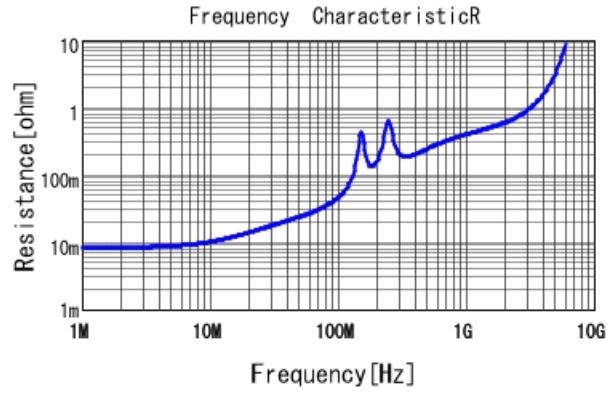
■ GRM3195C2A562JA01 R DCOV, 25degC
