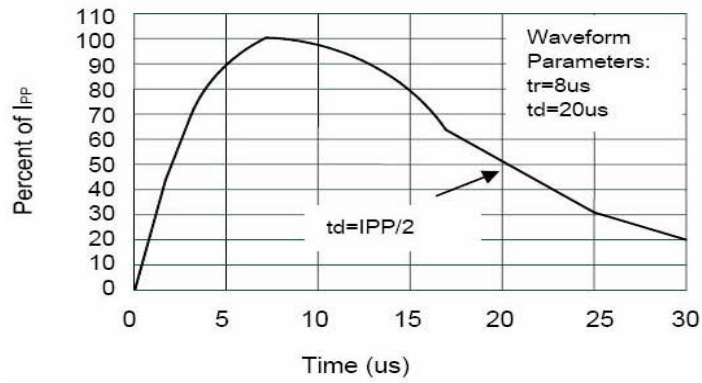
Pulse Waveform
