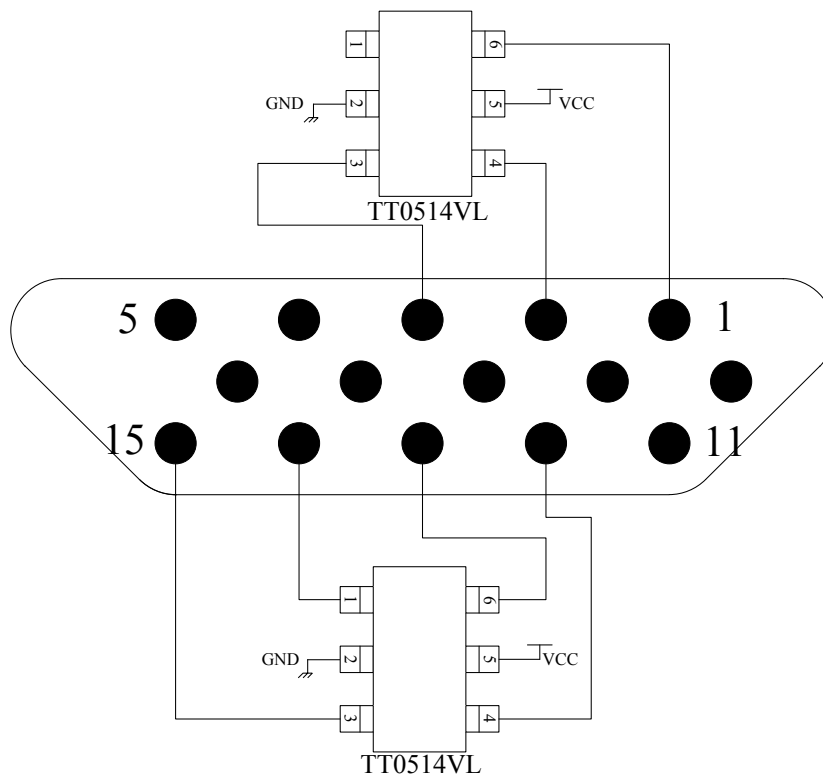
Layout Top View for Video (VGA) Interface with TT0514VL
