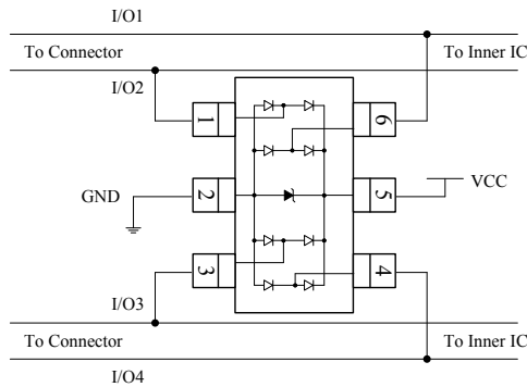
Figure 1 TT0514VL pin connection in PCB
