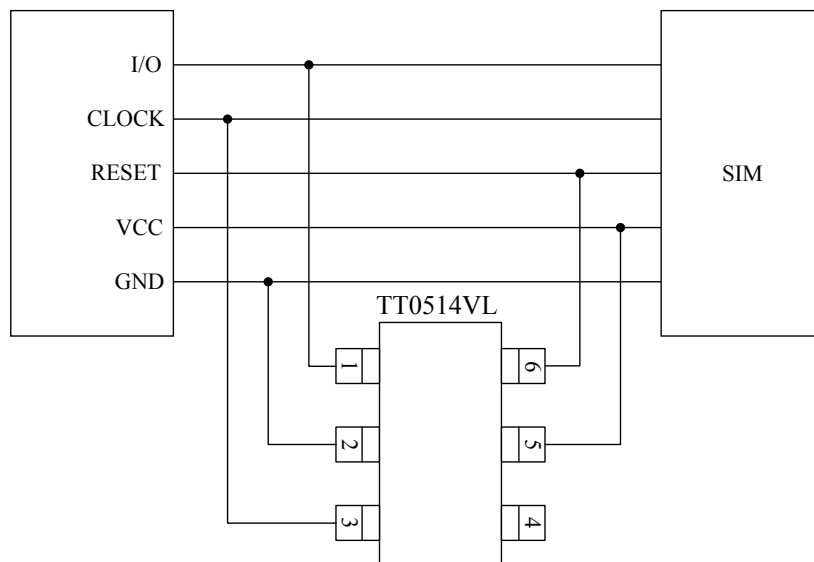
Layout Top View for SIM Port with TT0514VL
