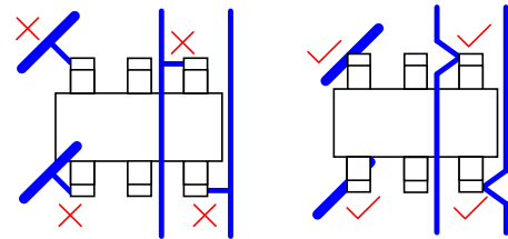
Figure 2 TT0514VL Layout Guideline
