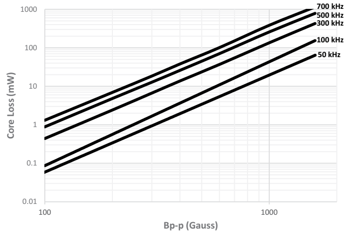
HCM1A0805V2-220-R
