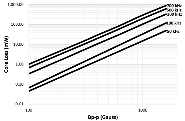
HCM1A0805V2-1R0-R
