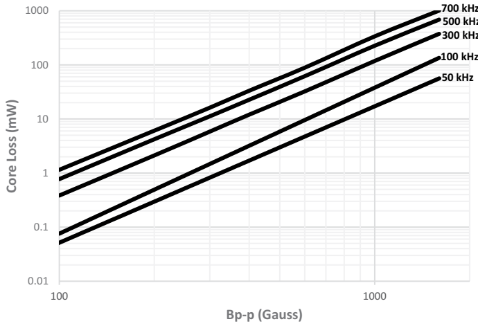
HCM1A0805V2-4R7-R
