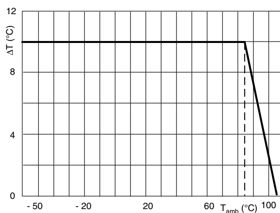
Max. allowed component temperature rise ( \Delta T ) as a function of the ambient temperature ( T_{amb} )
