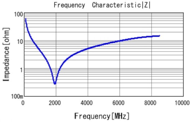
■ GRT0335C1H270FA02 |Z| DC0V, 25degC
