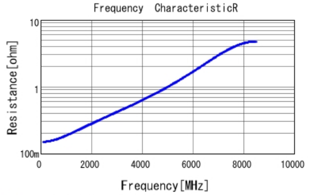
■ GRT0335C1H270FA02 R DC0V, 25degC
