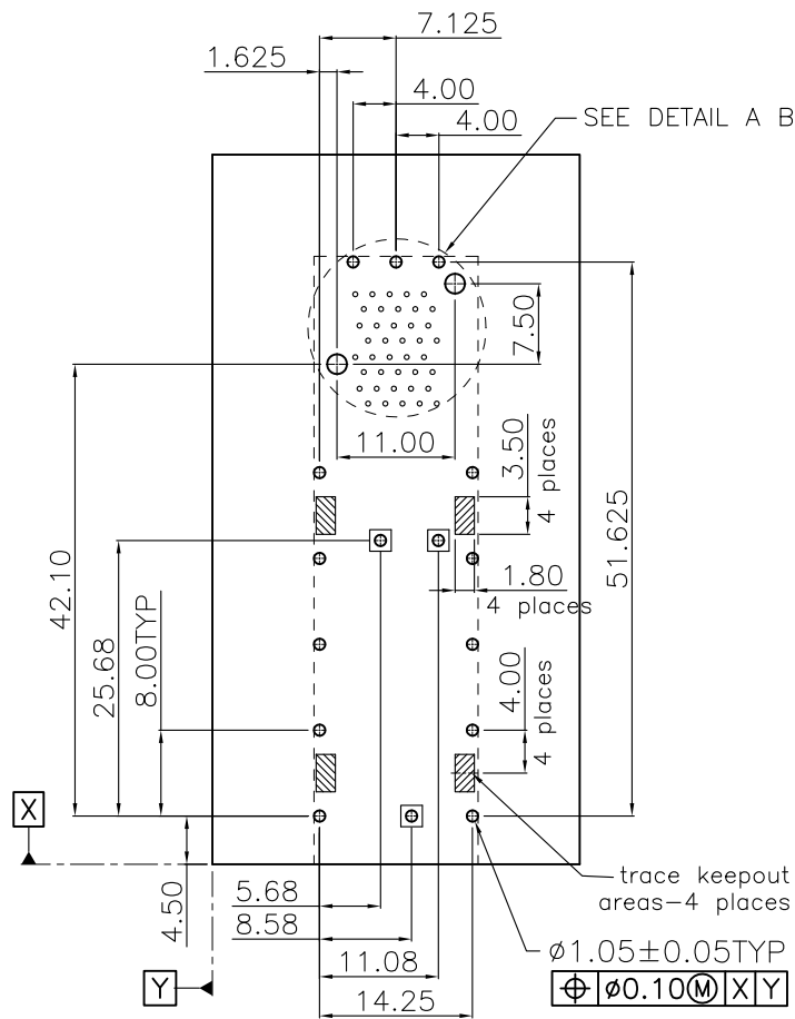
RECOMMENDED PCB LAYOUT AND PCB TOLERANCE \pm 0.05
