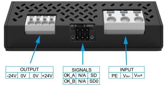
Fig. 11 Pin allocation of RCM300
