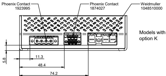
Fig. 9 Case of RCM300 (RCM02) weight approx. 820 g, Aluminum, EP-powder coated
