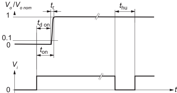
Fig. 6 Typical output response to V_i . If option M is not fitted, t_{hu} = 0 ms.
