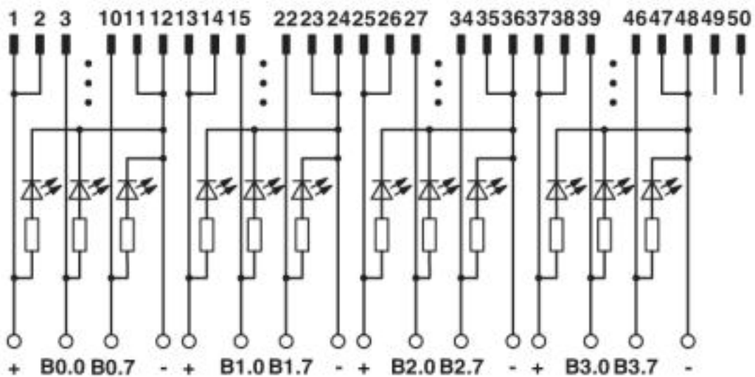
45-FLK50/LA/ZFKDS/PLC connection scheme
