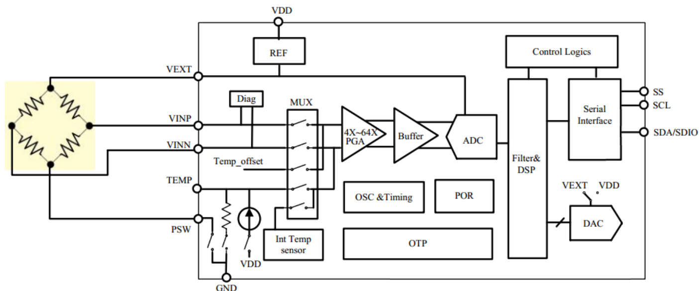
CPS121-700 BLOCK DIAGRAM
