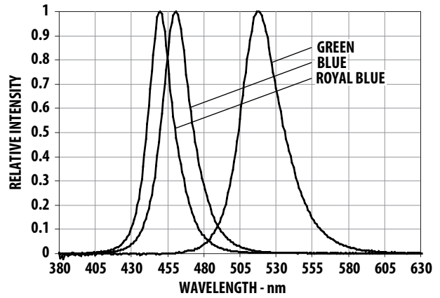
Figure 10. Relative Intensity vs. Wavelength for Blue, Royal Blue and Green.
