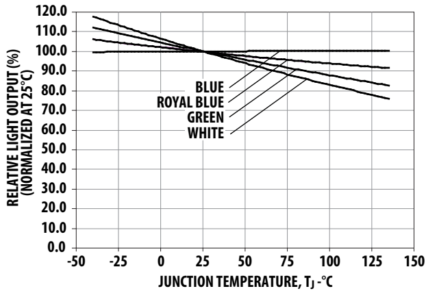
Figure 15. Relative Light Output vs. Junction Temperature.
