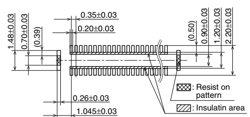
Recommended PC board pattern (TOP VIEW)
