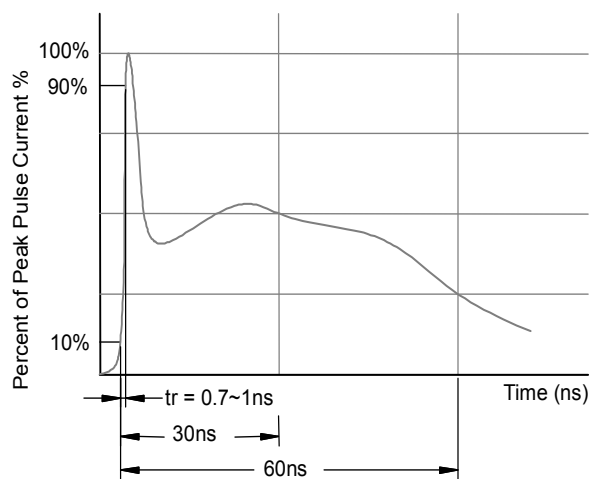
Fig 2. ElectroStatic Discharge (ESD) pulse waveform according to IEC 61000-4-2
