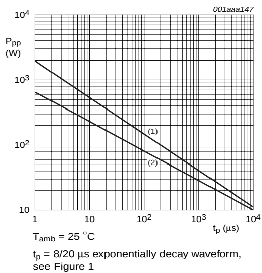
Fig 3. Peak pulse power dissipation as a function of pulse time; typical values
