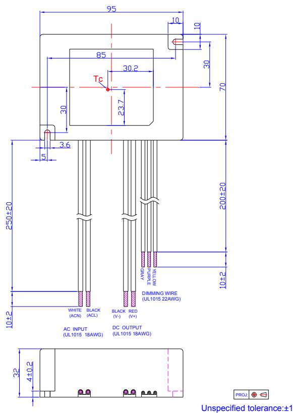
EUC-042SxxxDS
