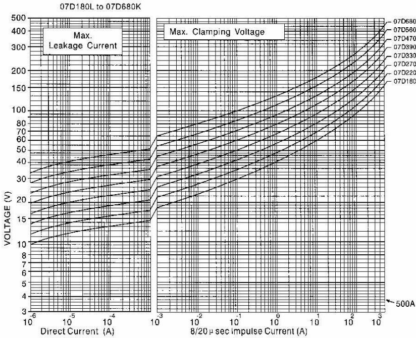
V-I curve
