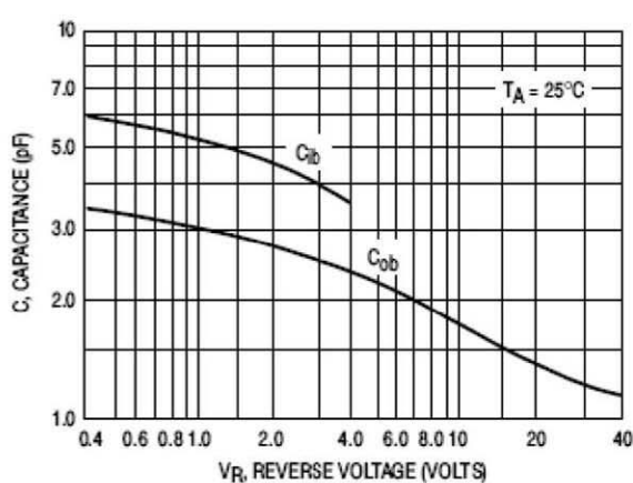
Figure 5. Capacitances
