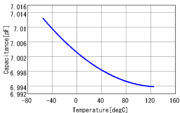
Temperature Characteristics
