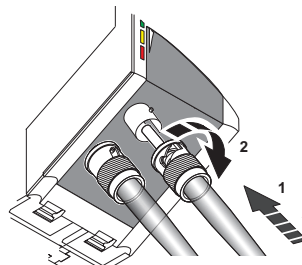
Figure 13 B-FOC connection
