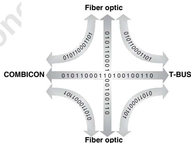
Figure 4 Communication between the interfaces
