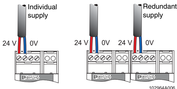
Figure 9 Individual/redundant supply
