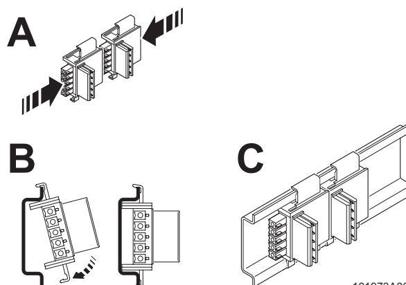
Figure 7 Combined assembly
