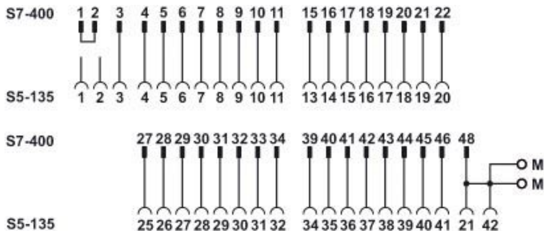
Connection diagram
