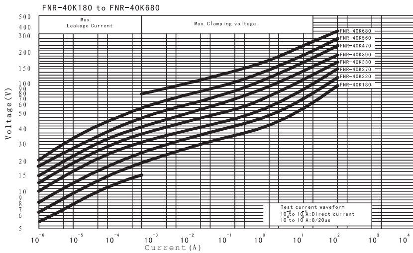
V-I Curve
