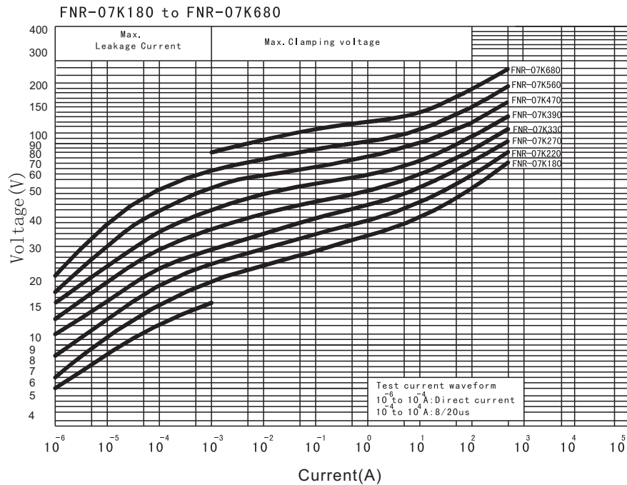
V-I Curve
