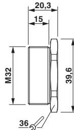
Dimensional drawing
