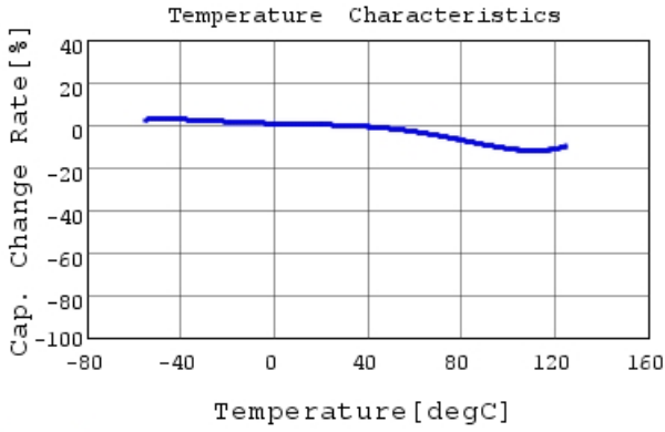
GRM55ER72A475KA01 C-Temp. capchange, DC0.0V,
