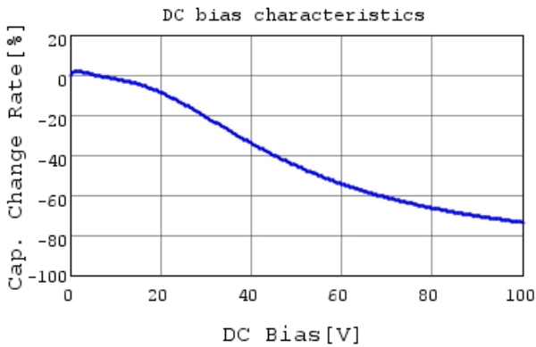
GRM55ER72A475KA01 C-DC bias capchange, 25.0c
