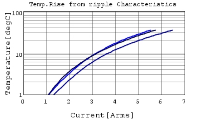
GRM55ER72A475KA01 Temp.rise 100kHz
