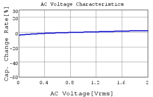
GRM55ER72A475KA01 C-AC Voltage capchange, Dc
