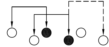
SCHEMATIC (NON-SHORTING)
