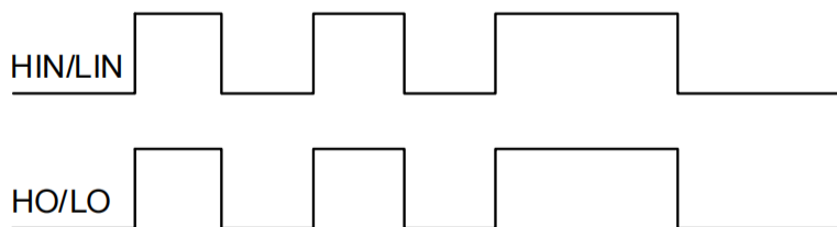
Figure 5. FAN7382MX Input and output timing waveform
