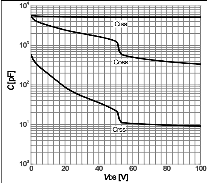
Diagram 13: Typ. capacitances
