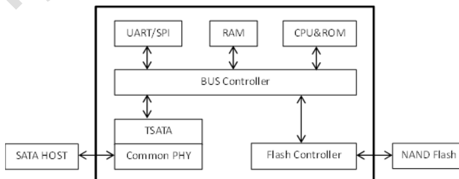
[Figure 1-1] SSD Functional Block Diagram
