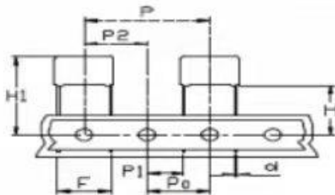
Fig 3 Pitch: 10/12.5/15 Po=12.7
