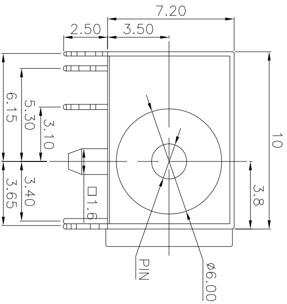
P.C.B LAYOUT(copper-sided view) 11.25
