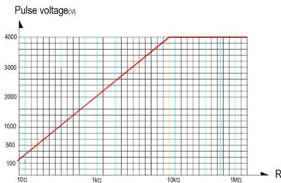
Pulse load rating in accordance with IEC 60115-1,4.27; 1.2μs/50μs ; 5 pulses loaded, for permissible resistance change < \pm(0.5\%+0.05\Omega)
