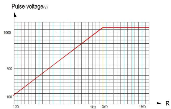
Pulse load rating in accordance with IEC 60115-1,4.27; 10μs/700μs ; 10 pulses loaded, for permissible resistance change < \pm(0.5\%+0.05\Omega)
