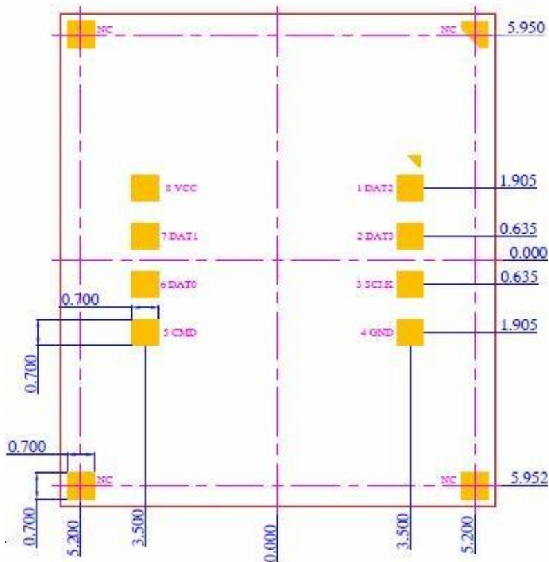
Figure 2: Bottom View (Unit:mm)
