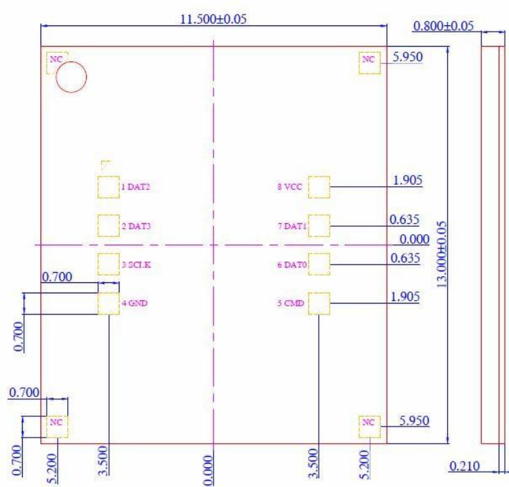
Figure 1: Top View and Side View (Unit:mm)
