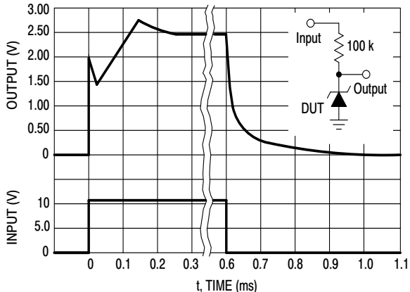
Figure 13. Response Time
