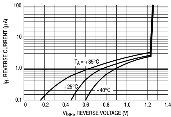
Figure 2. Reverse Characteristics
