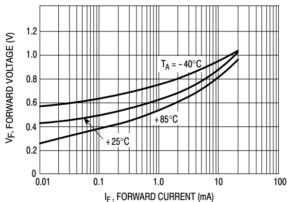
Figure 10. Forward Characteristics
