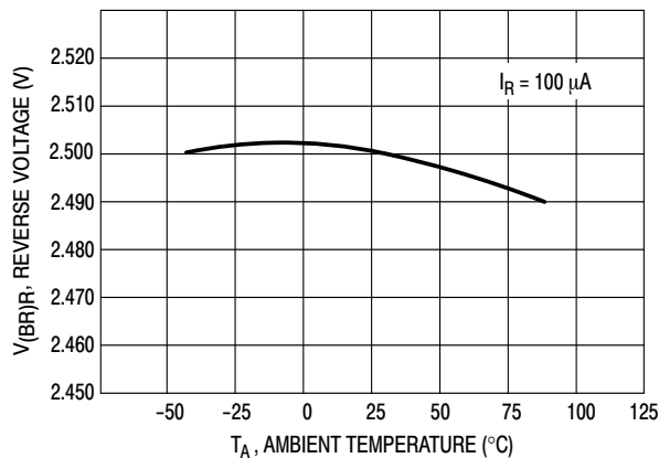
Figure 11. Temperature Drift
