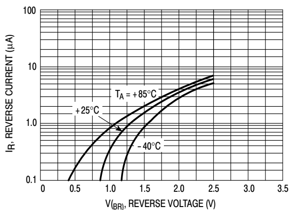
Figure 8. Reverse Characteristics
