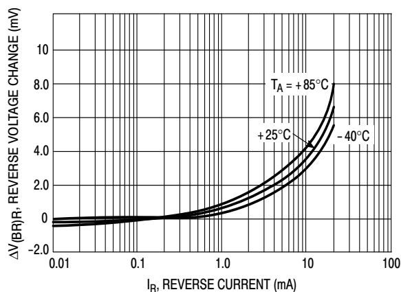
Figure 9. Reverse Characteristics
