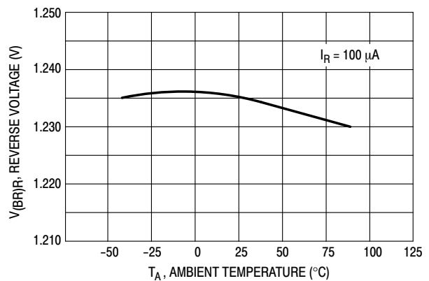
Figure 5. Temperature Drift
