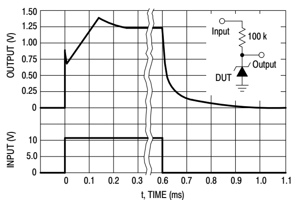
Figure 7. Response Time
