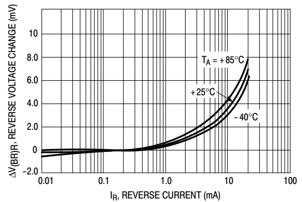
Figure 3. Reverse Characteristics
