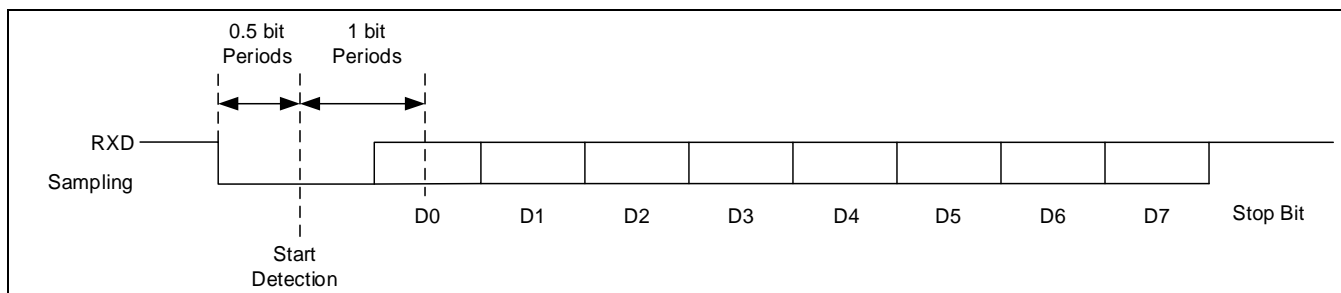
Figure 13-3 接收数据
