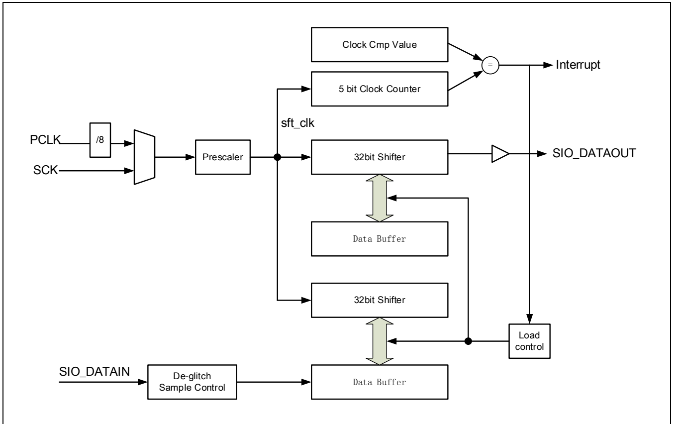
Figure 22-1 SIO模块框图
