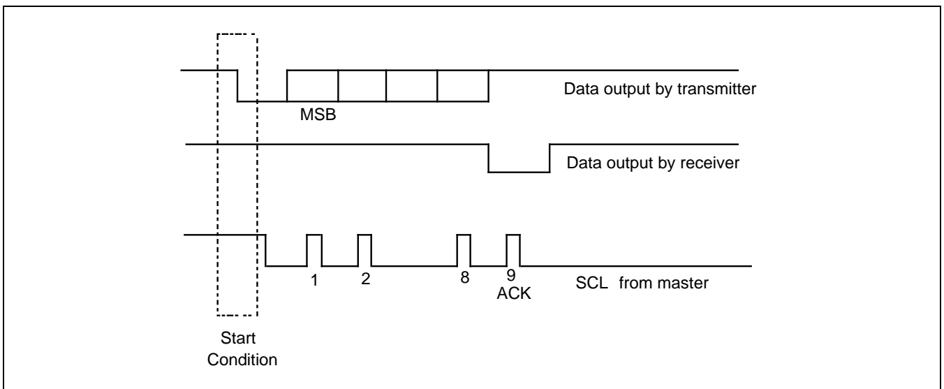
Figure 20-5 应答
