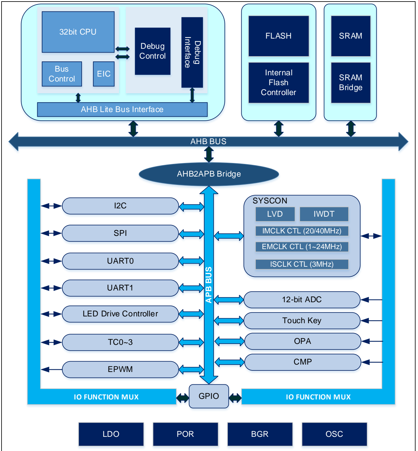
Figure 1-1 APT32F171模块框图
