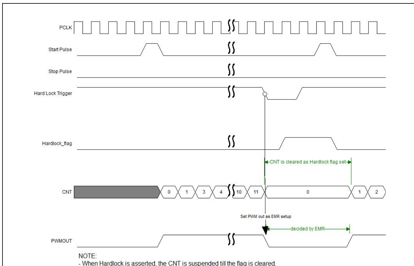
Figure 16-12 Hard Lock
