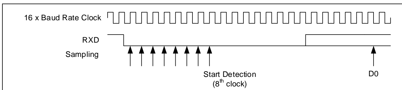
Figure 13-2 起始位检测
