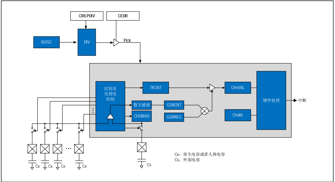
Figure 23-1 Touch Sensor模块框图
