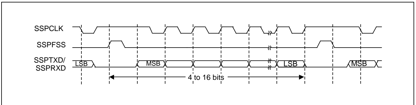
Figure 21-6 Motorola SPI 帧格式 (连续传输), SPO = 1 和 SPH = 0
