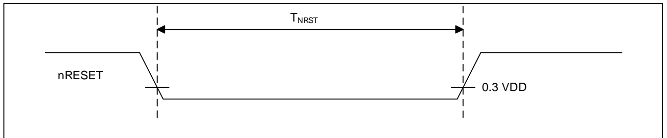
Figure 24-1 nRESET 输入时序
