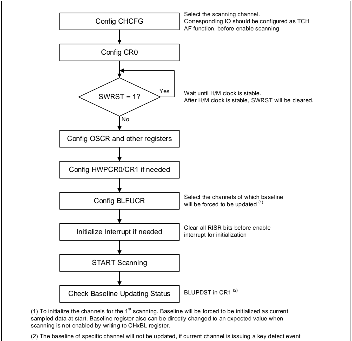
Figure 23-3 软件配置流程
