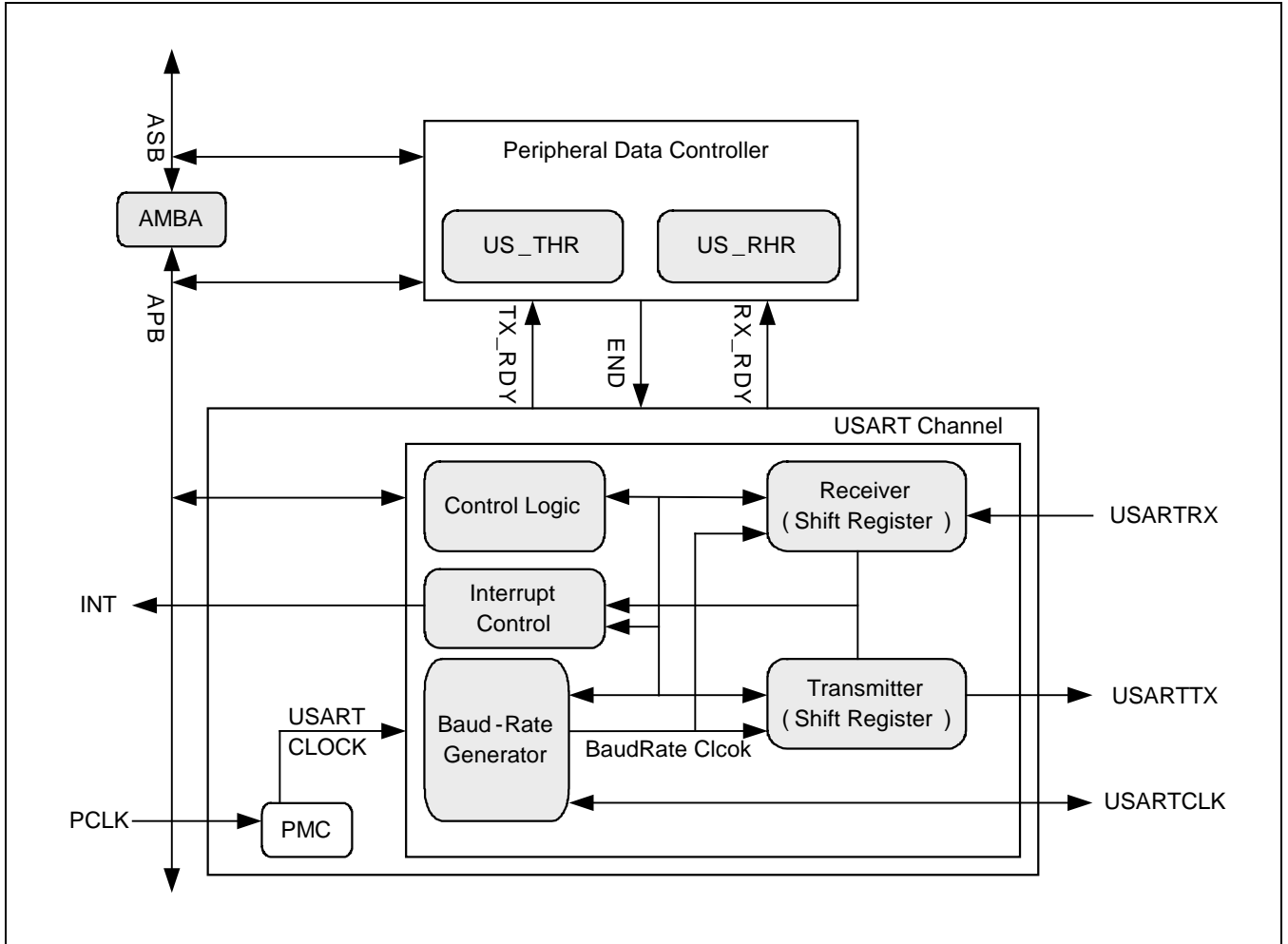
Figure 18-1 USART模块框图
