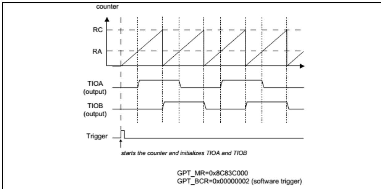
Figure 12-10 2 Square Signals
