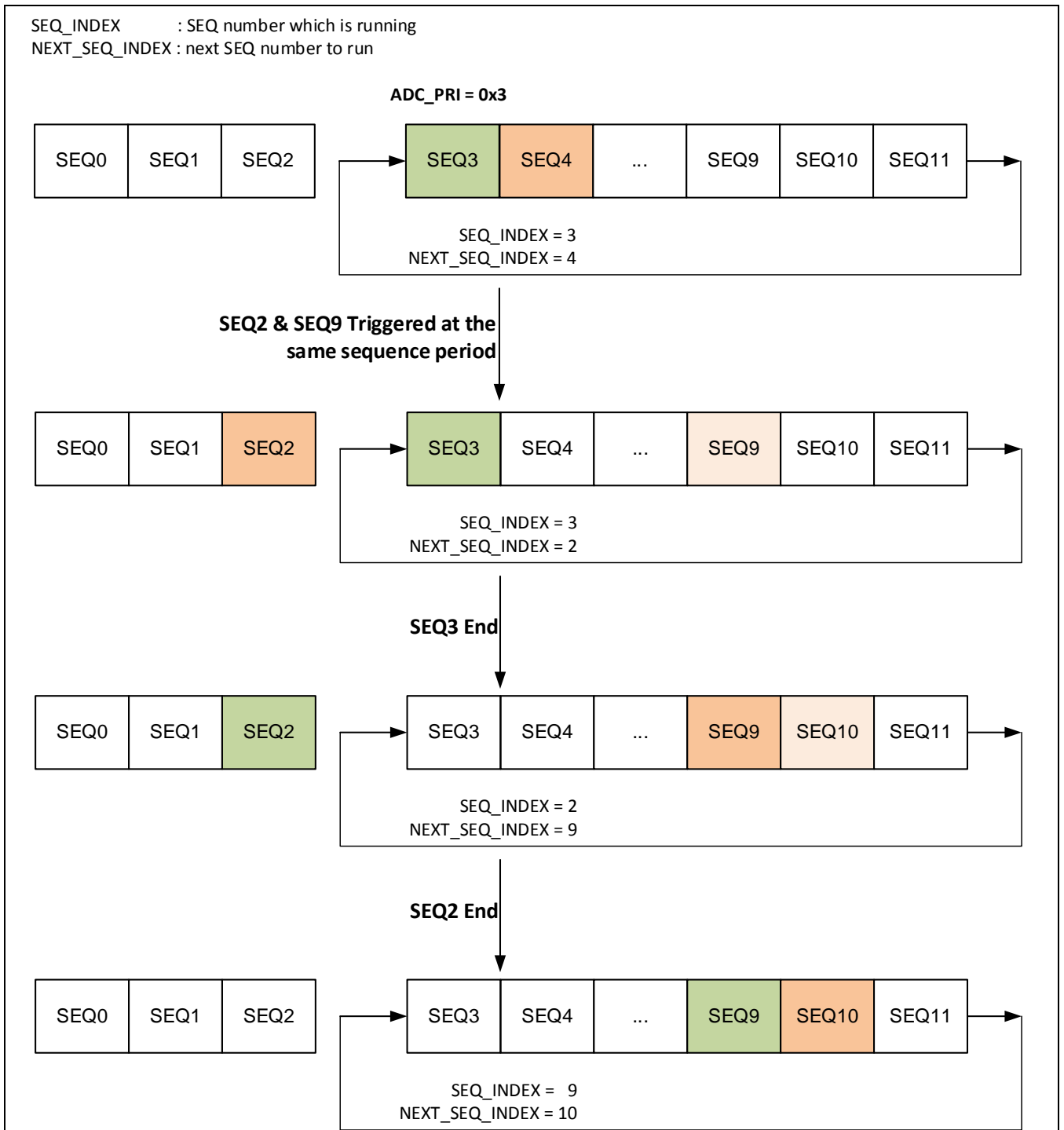
Figure 8-7 触发优先级示意图
