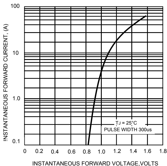
FIG.4-TYPICAL FORWARD CHARACTERISTICS
