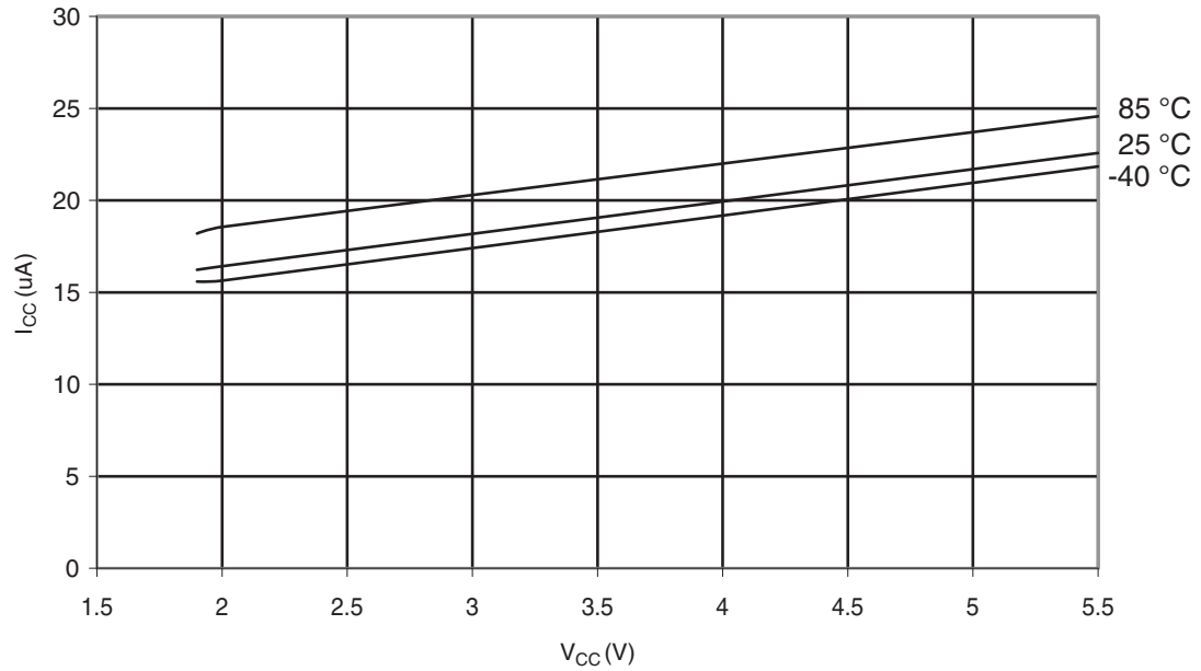
Figure 31-327. ATmega328: Brownout Detector Current vs. V_{CC}
