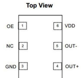
Figure 1. Pin Assignments
