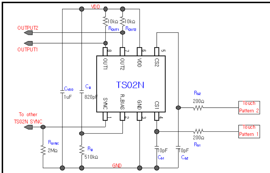
TS02N Application Example Circuit
