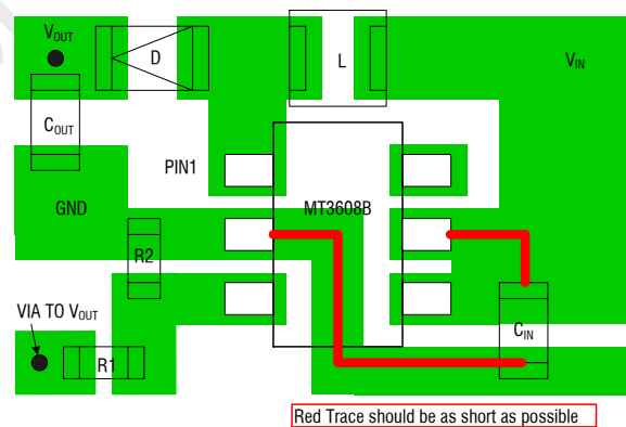
Figure 3. MT3608B Suggested Layout
