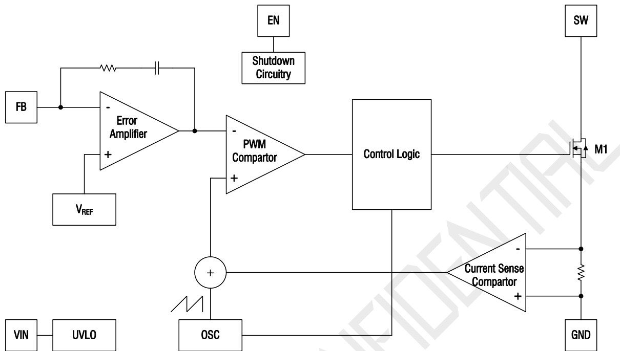
Figure 2. MT3608B Block Diagram
