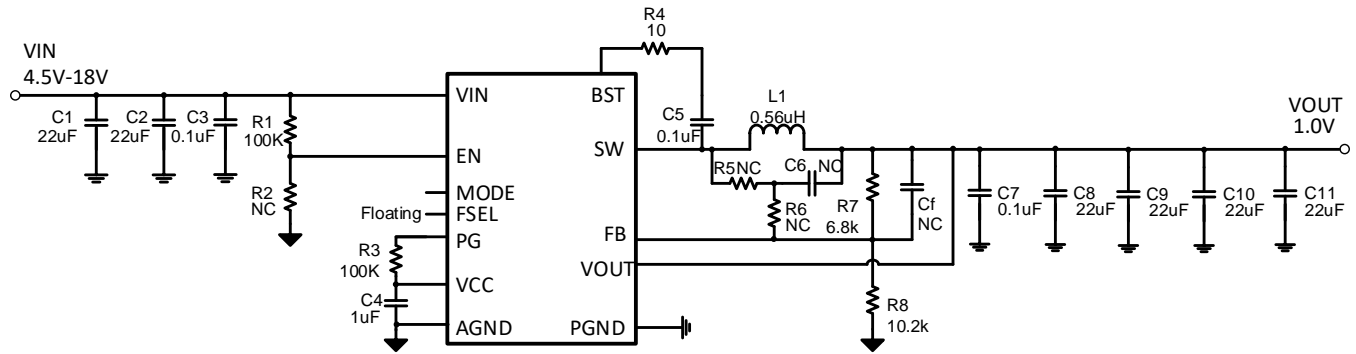
Figure 10. SCT2260C Design Example, 1.0V Output
