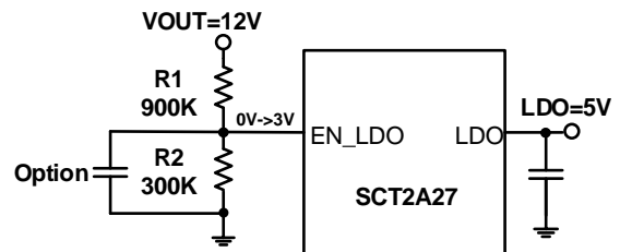
Figure 15. Resistor divider set 5V LDO output
