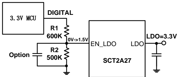
Figure 10. 3.3V Digital signal set 3.3V LDO output,
