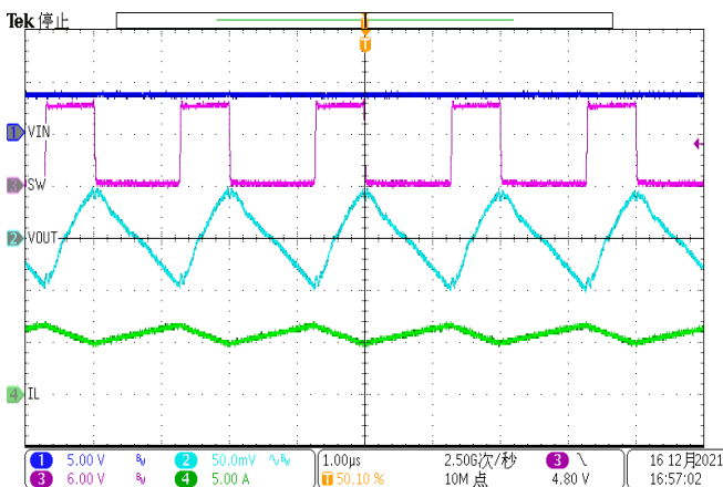
Figure 19. Steady state (Iload=2A)
