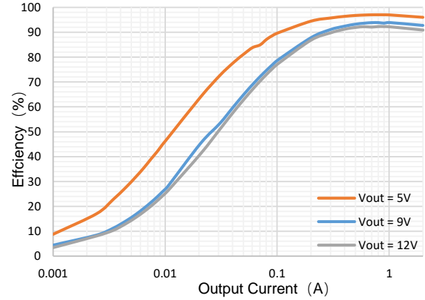
Figure 2. SCT1270F Efficiency vs Load Current, Vin=3.6V
