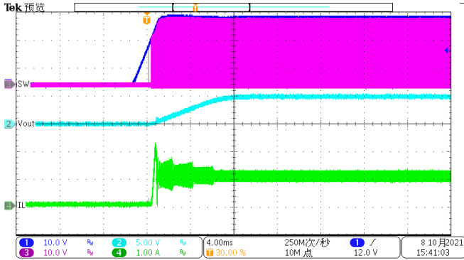
Figure 11. Power up(Iload=1A)
