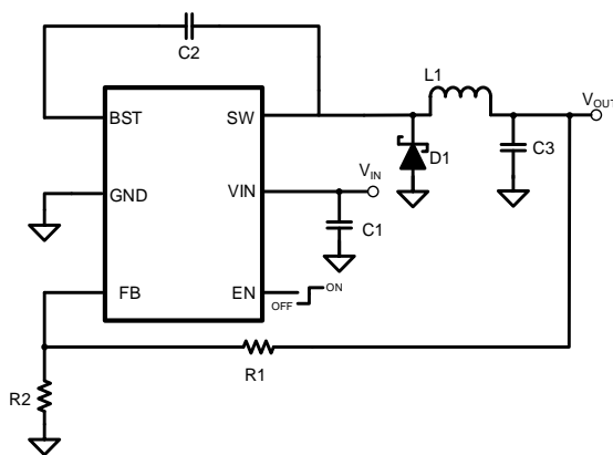
4.5V-60V, Asynchronous Buck Converter
