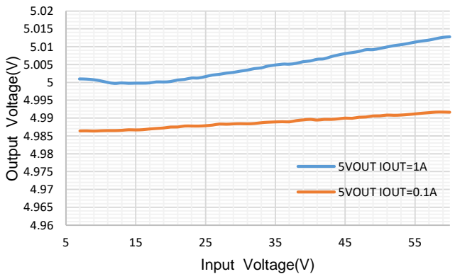
Figure 6. Line Regulation
