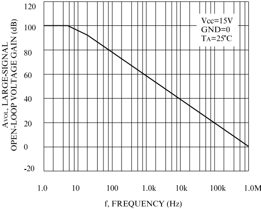
Figure 2. Open-Loop Frequency
