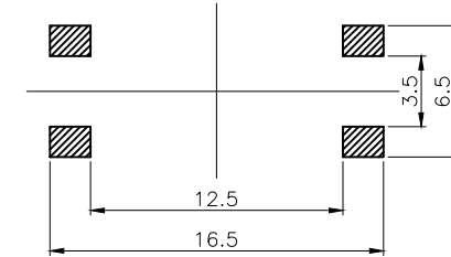
PCB. WELDING DRAWING
