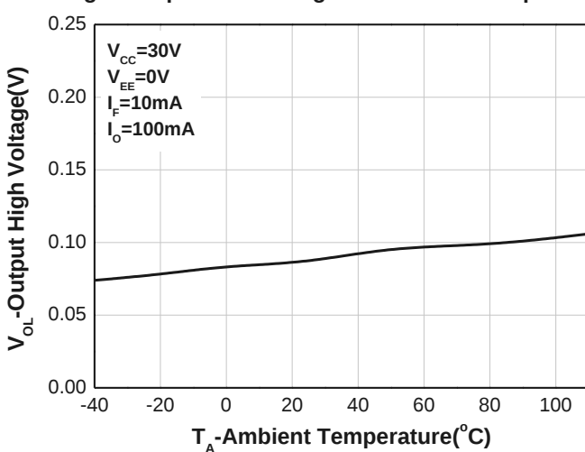
Fig. 5 Output Low Voltage vs. Ambient Temperature
