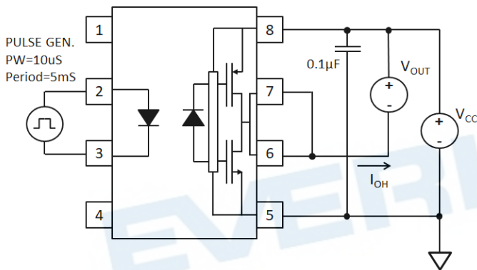
Fig. 15 I_{OH} Test circuit
