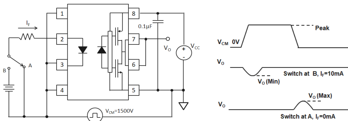
Fig. 22 CMR Test circuit
