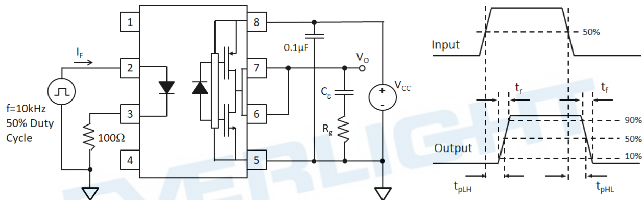
Fig. 21 Switching Time Test circuit
