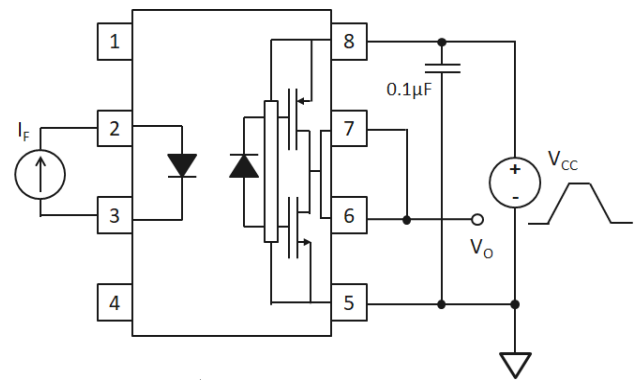
Fig. 20 UVLO Test circuit
