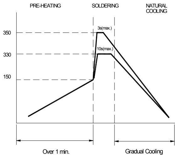
Figure 2. Hand Soldering
