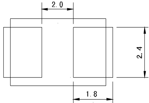
suggested solder pad layout
