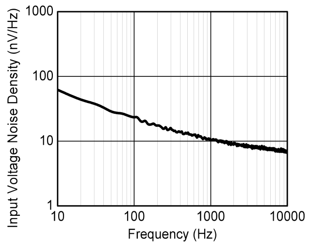
Noise Density
