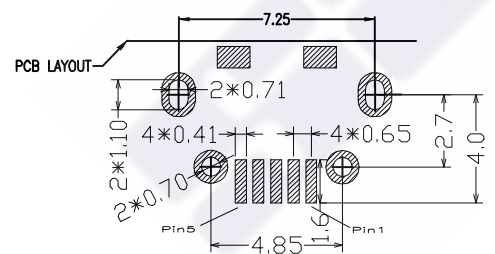
RECOMMENDE.P.C.B LAYOUT(TOP VIEW) EFAULT YOLERANCE:±0.05
