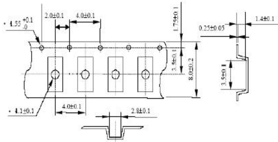
8.3. Reel dimension &amp; Outline drawing
