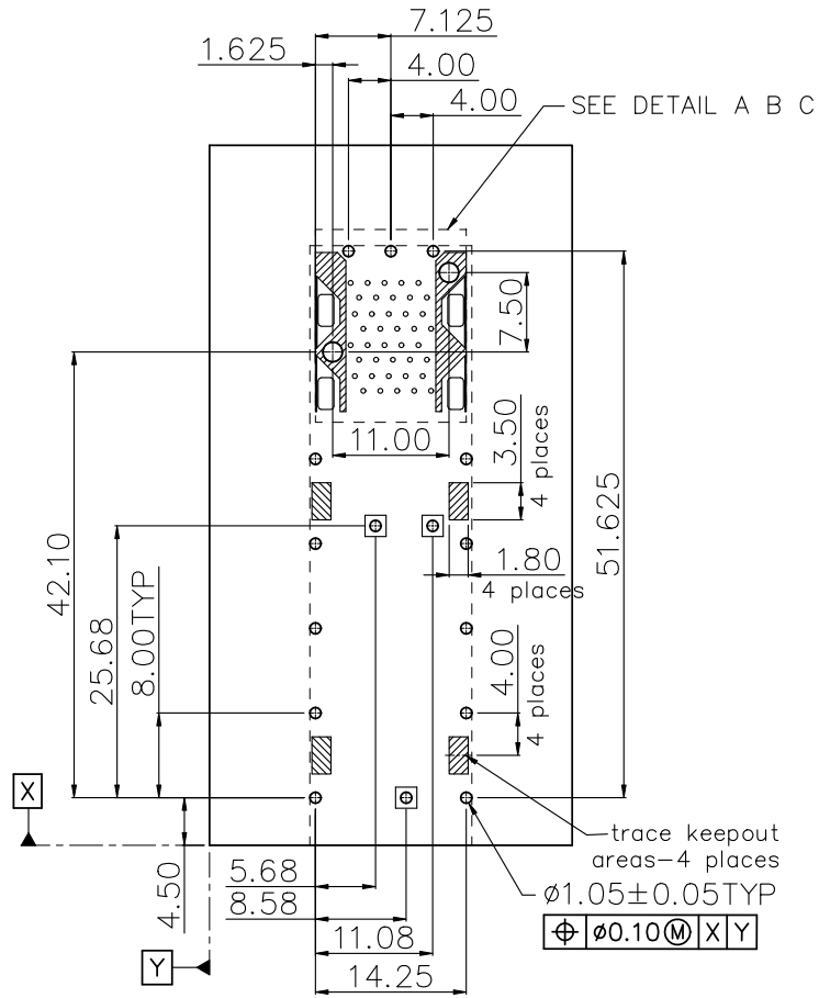
RECOMMENDED PCB LAYOUT AND PCB TOLERANCE ±0.05
